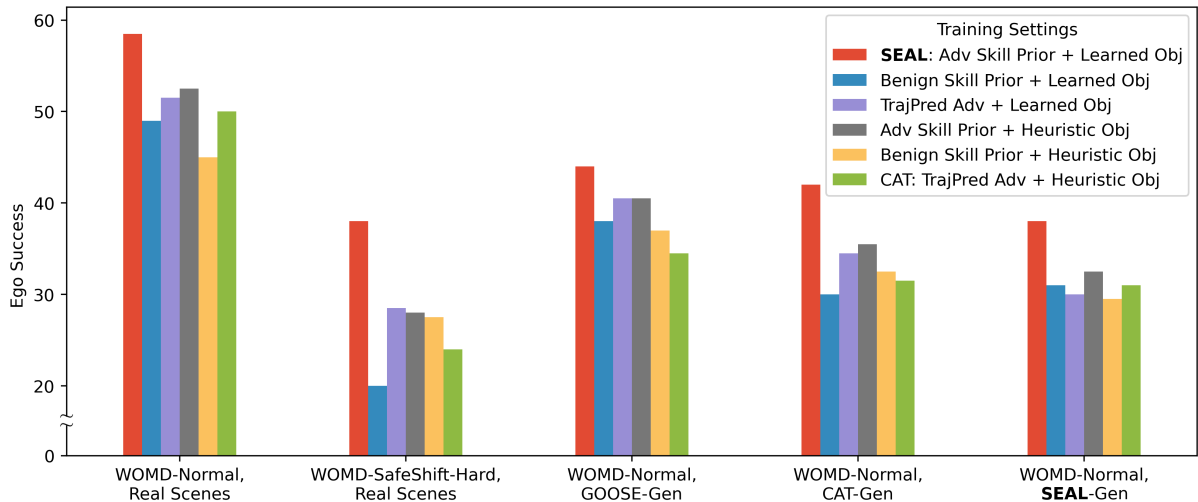
Fig. 3: Ablation study on SEAL scenario generation training pipelines. Our full approach with learned objectives (Section IV-A) and adversarial skill policies (Section IV-B) produces the strongest downstream agents, across all five evaluation settings.
