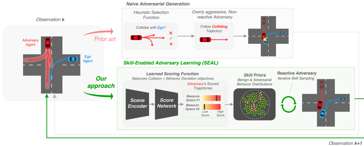
Fig. 1: An overview of SEAL. Our scenario generation approach leverages a learned scoring function and a reactive, adversarial skill policy, for improved adversary realism and closed-loop training, leading to safer autonomous driving agents.
