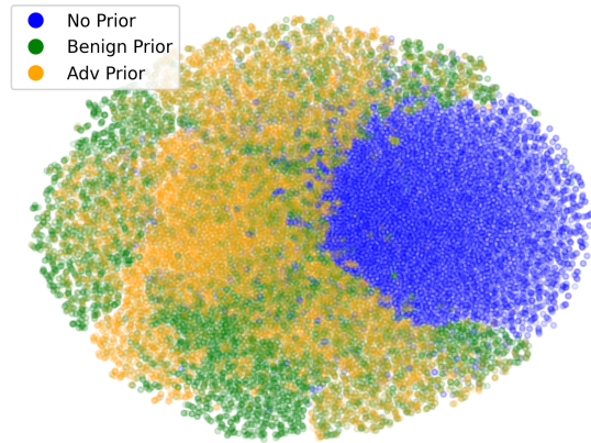
Fig. 2: Skill-space visualized with t-SNE [46]. Benign and adversarial priors map to several regions representing useful, human-like skills, with meaningful separation and overlap.
